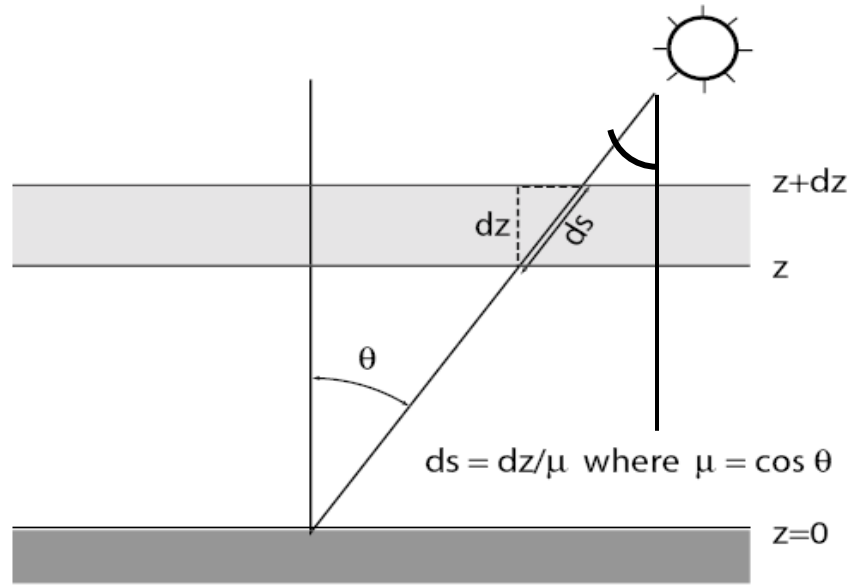
Figure 3. Relationship between slant and vertical paths in a plane parallel atmosphere. This approximation ignores horizontal variations in the structure of the atmosphere and assumes all relevant radiative properties depend strictly on the vertical ( z ) direction. In addition, the curvature of the Earth is ignored assuming a ray of light (or a laser beam) does not propagate at very oblique angles, similar to ATL engagements (Petty, 2006). Note that alternate interior angles are congruent.
