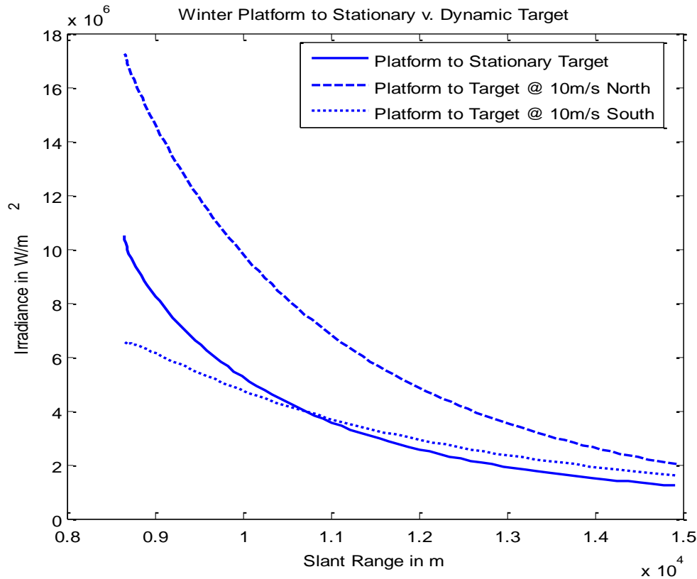
Figure 21. HELEEOS winter thermal blooming effects. Aircraft is northbound with a velocity of 50m \cdot s^{-1} . Peak irradiance curve is greatest when the platform and target move in the same direction. Peak irradiance curves for platform to stationary and southbound target intersect at a specific slant range due changes in thermal blooming effects. Within that specific slant range (occurring at approximately 10.75km in the figure) the peak irradiance becomes less for the southbound than the stationary target due to greater thermal blooming effects. There are no clouds or rain present during this engagement.
